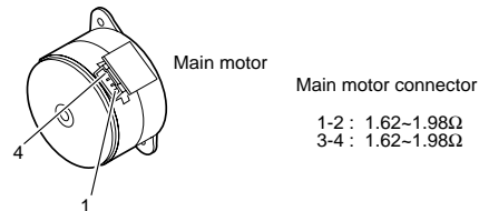
Figure 3-4 Main Motor Connector
