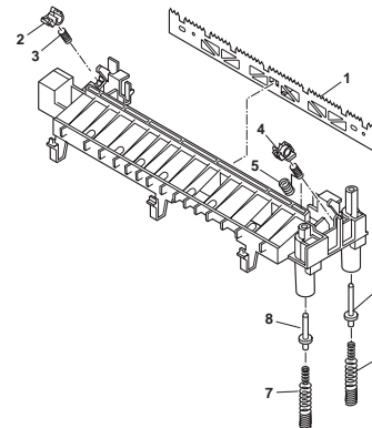
FIGURE 19 TRANSFER BLOCK ASS'Y
