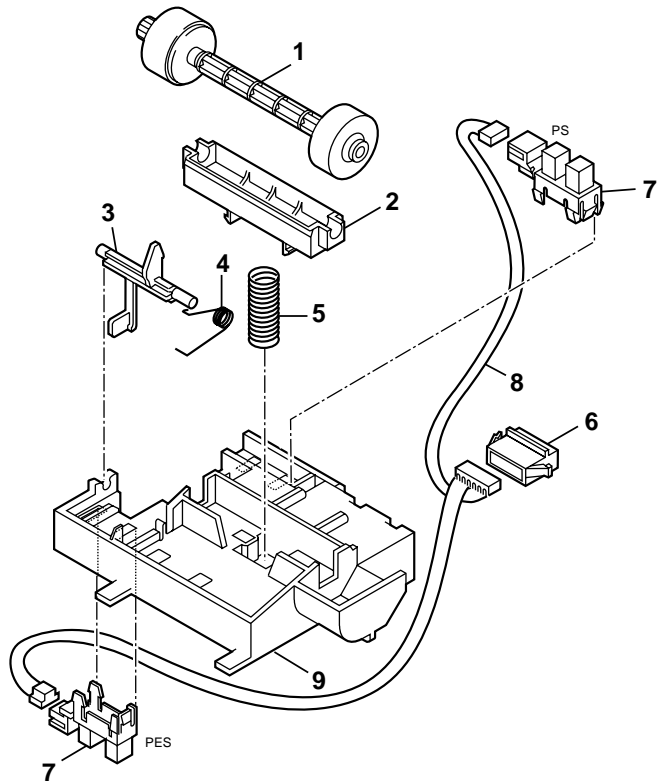
FIGURE 17 FEEDER ASS'Y
