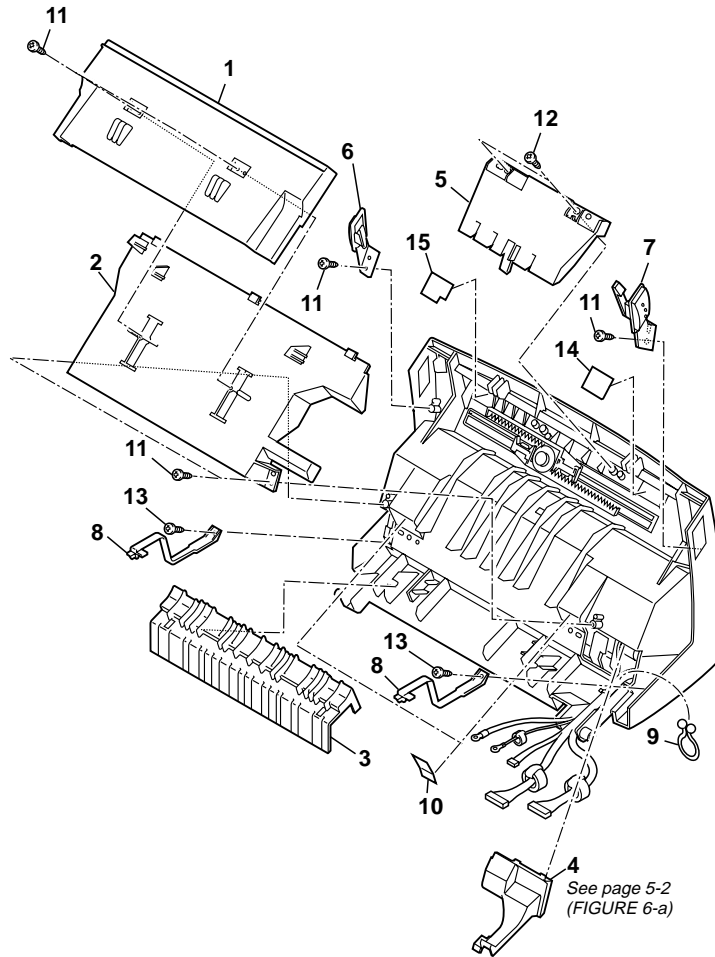
FIGURE 6 READING ASS'Y 1
