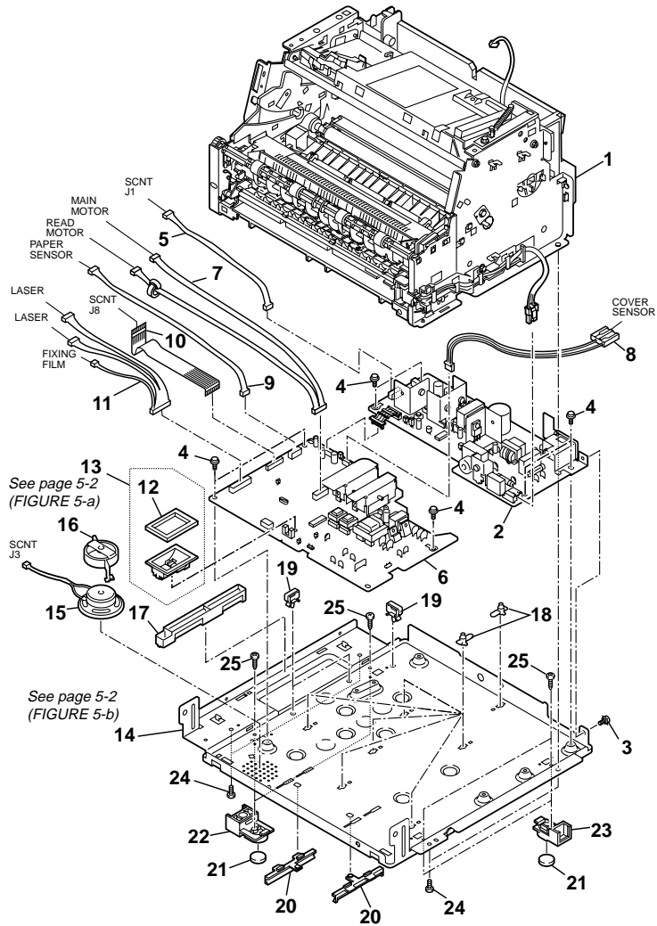
FIGURE 5 CIRCUIT BOARDS & BOTTOM PLATE
