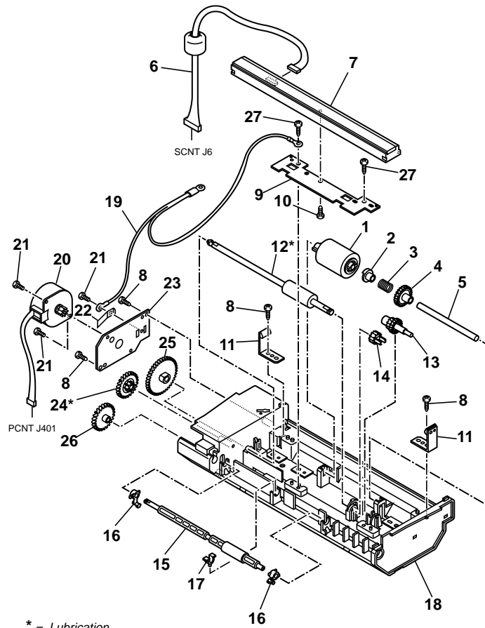
FIGURE 9 ADF LOWER
