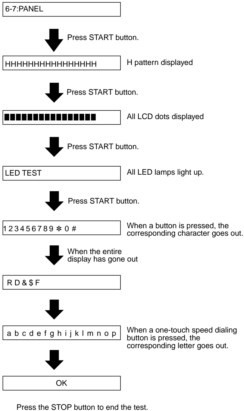
Figure 3-24 Operation Panel
