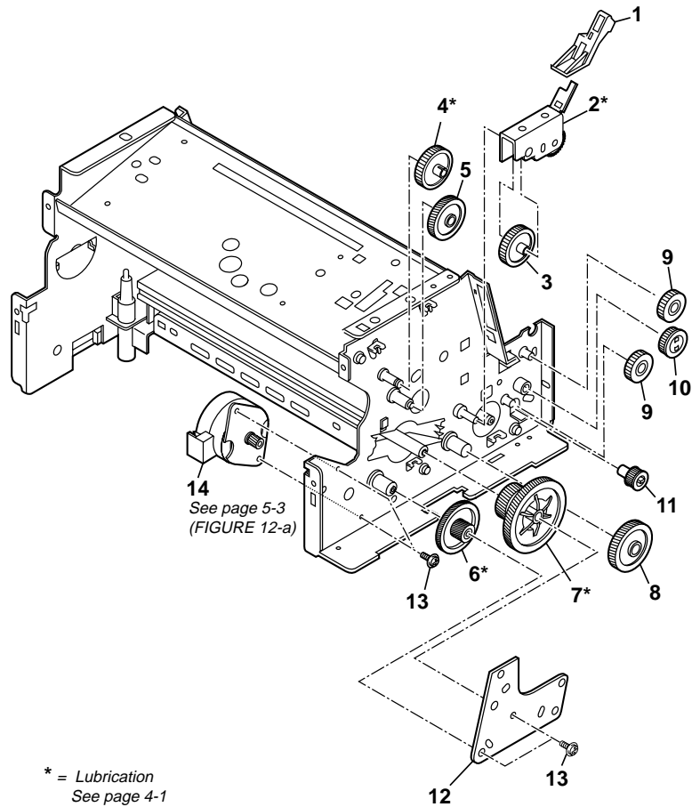
FIGURE 12 DRIVE GEARS
