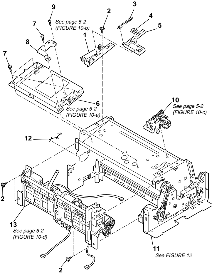
FIGURE 10 SCANNER ASS'Y
