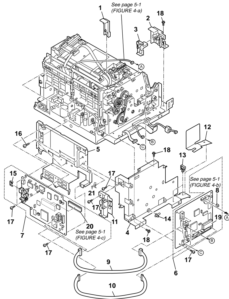
FIGURE 4 CIRCUIT BOARDS & MAIN FRAME
