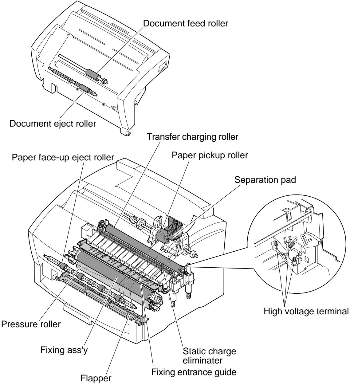
Figure 3-2 Cleaning Location 2
