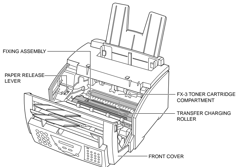
Figure 1-3 External View (1)
