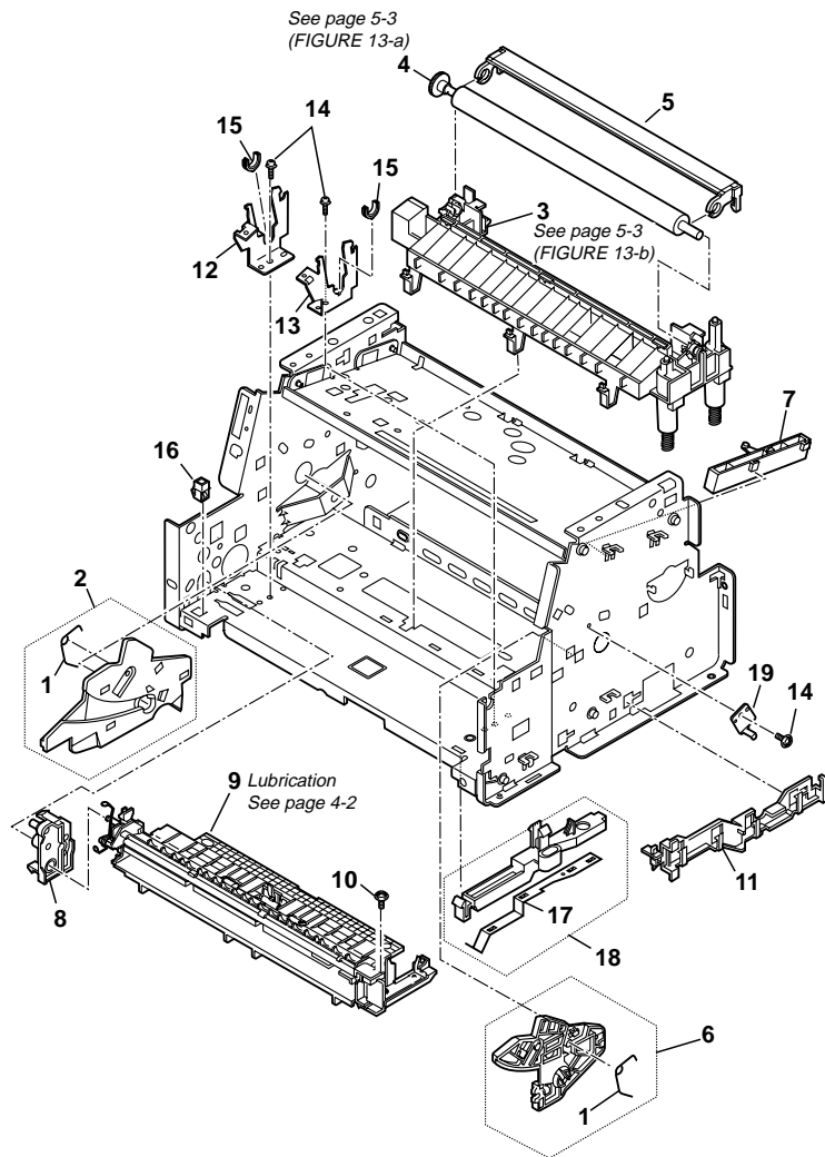
FIGURE 13 FIXING SECTION 2
