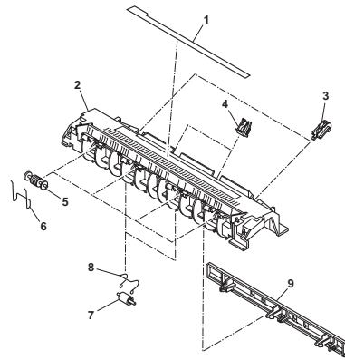
FIGURE 18 DELIEVRY ASS'Y
