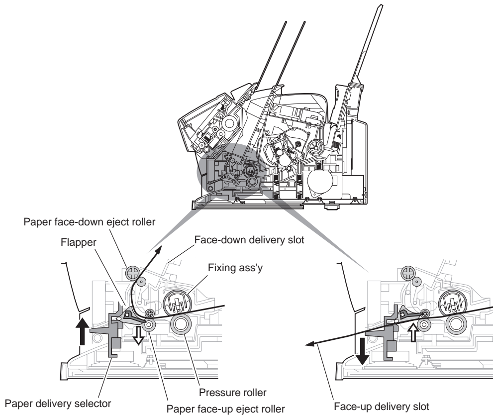
Figure 2-6 Paper Delivery Slot Switching
