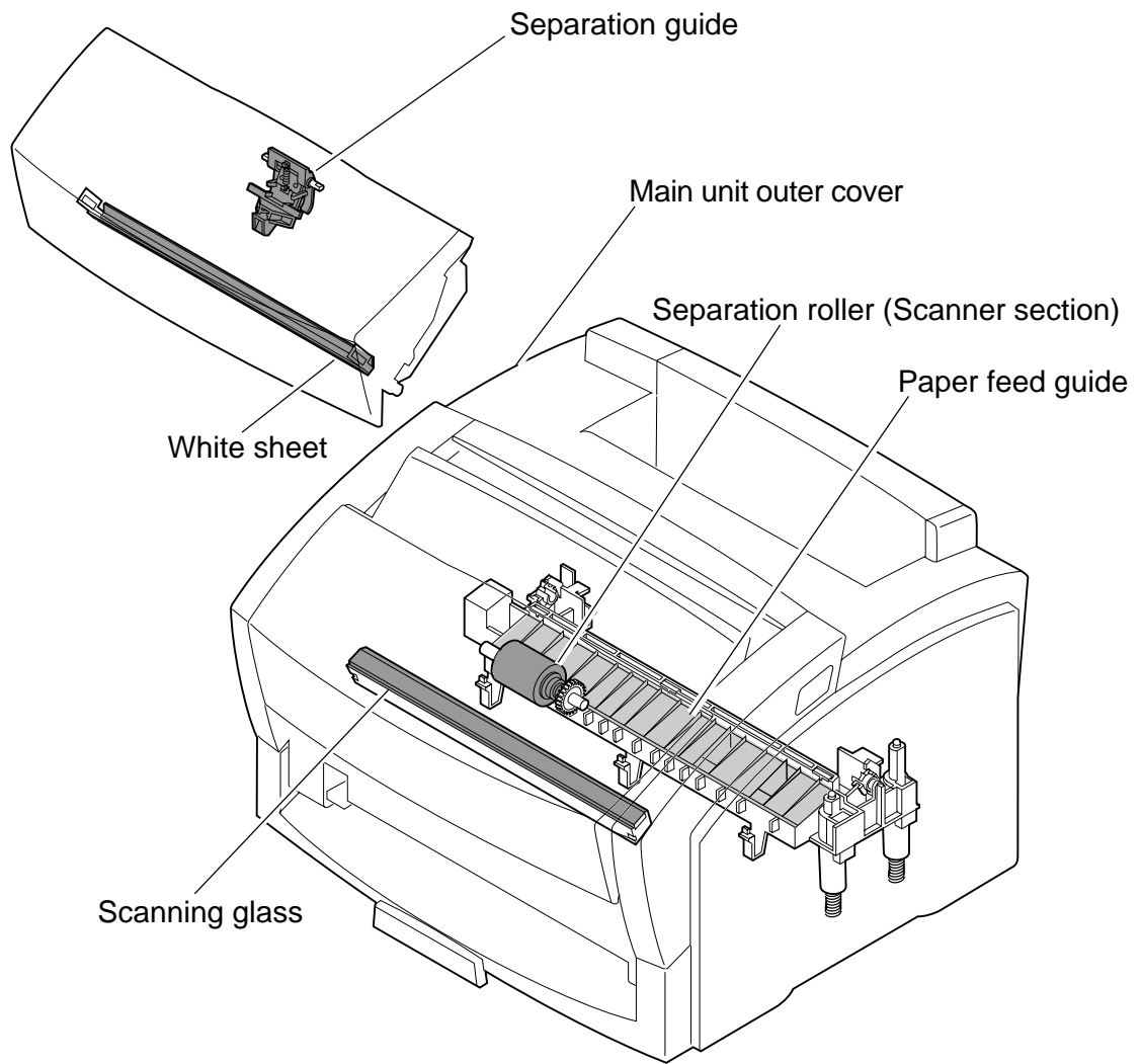
Figure 3-1 Cleaning Location 1
