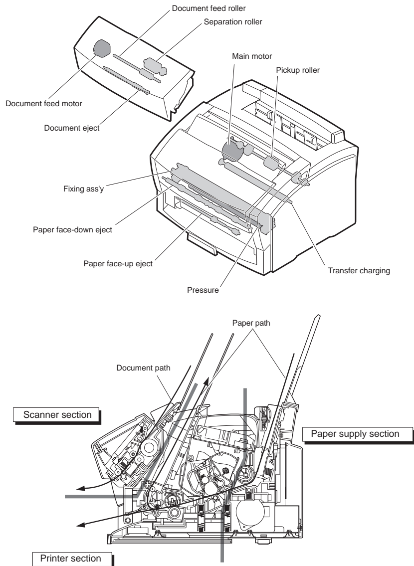
Figure 2-1 Drive System Layout
