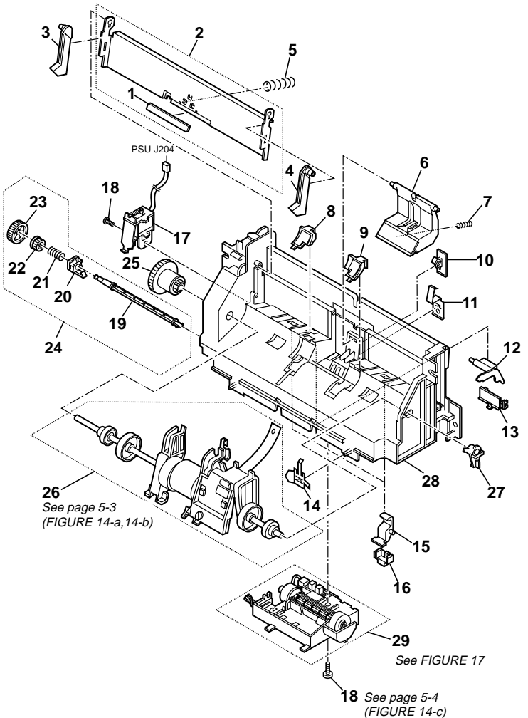
FIGURE 14 PAPER FEED SECTION
