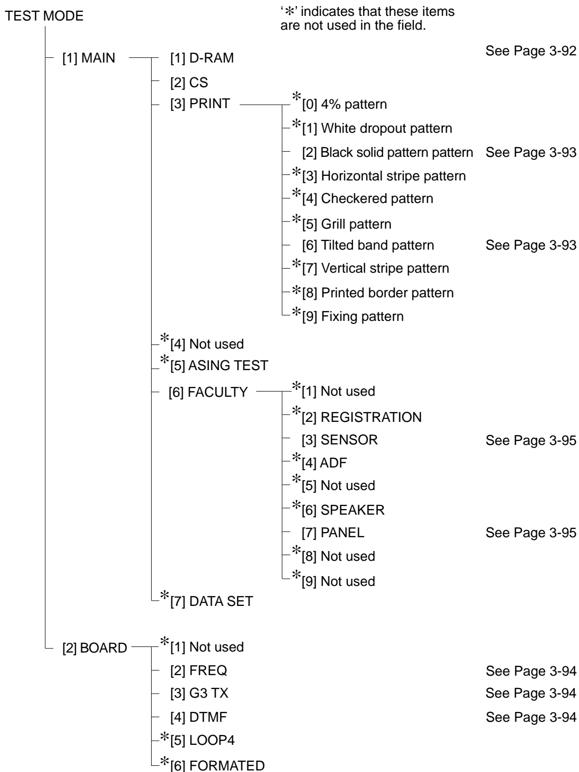
Figure 3-20 Test Mode
