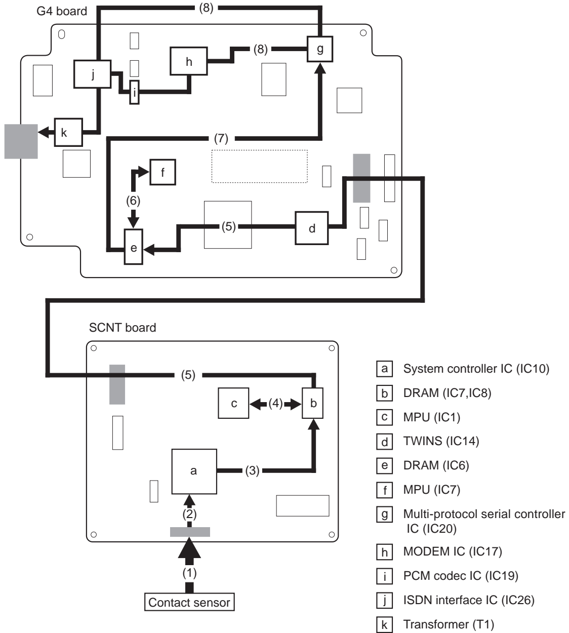
Figure 2-9 Transmission Image Signal Flow
