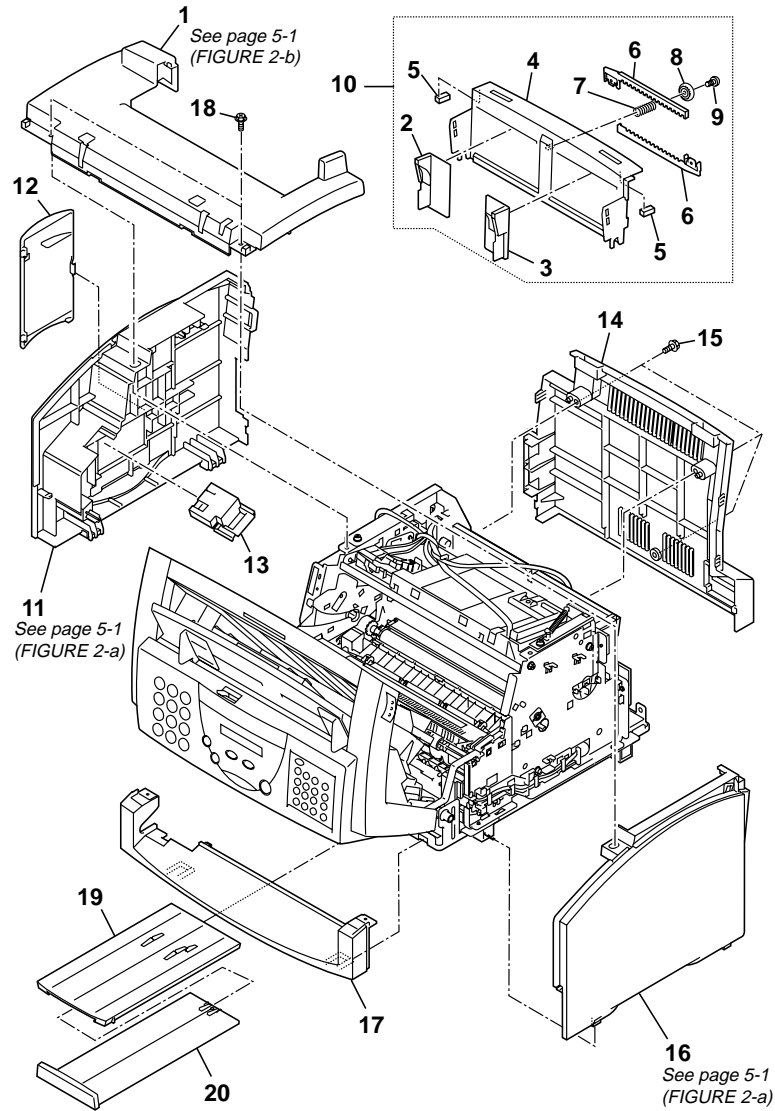
FIGURE 2 COVERS & TRAY ASS'Y
