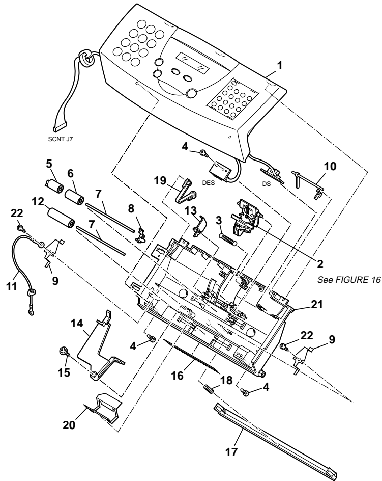
FIGURE 8 OPERATION PANEL ASS'Y & ADF UPPER
