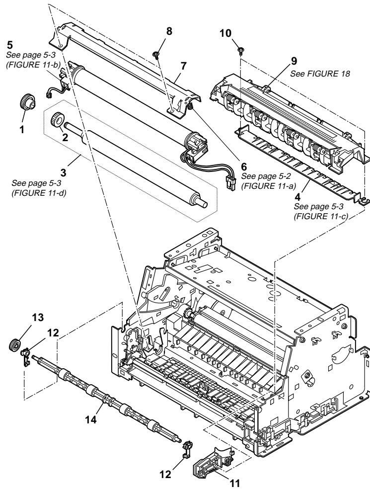
FIGURE 11 FIXING SECTION 1
