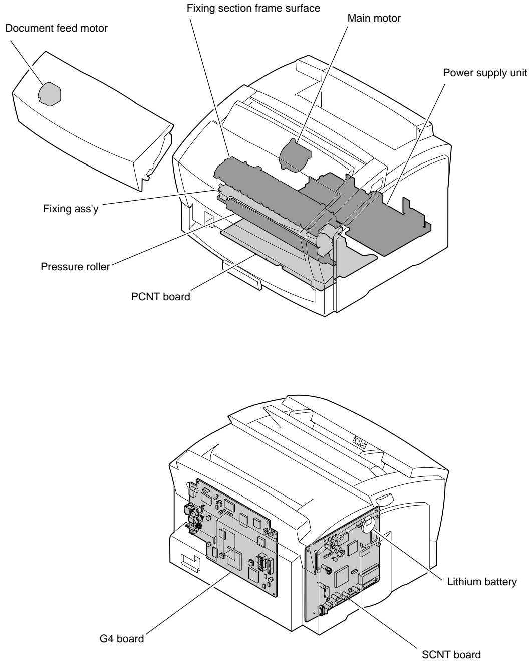
Figure 1-9 Personnel Hazards (1)
