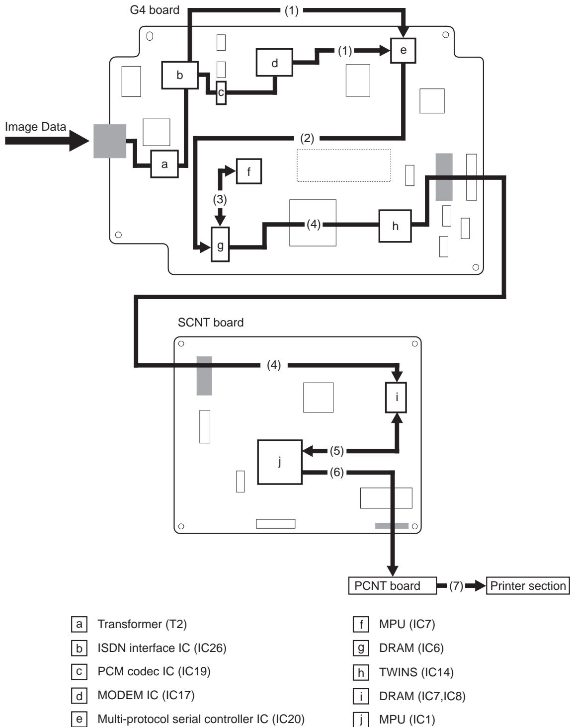
Figure 2-10 Reception Image Signal Flow
