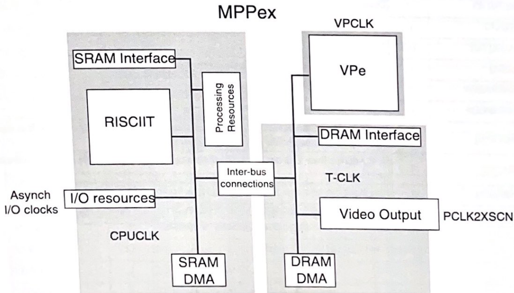
Figure 18. The MPPex Clock Distribution
