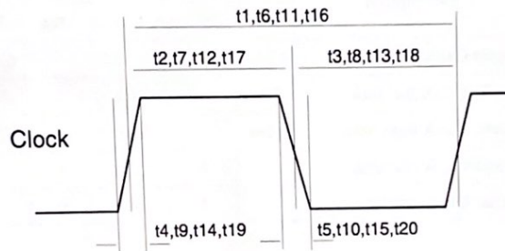
Figure 20. Clock Timing Diagram
