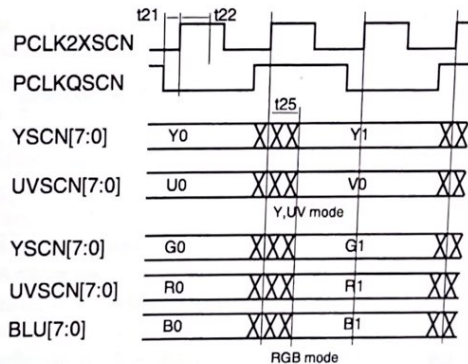
Figure 4. 2x Clock Video Out Bus Timing
