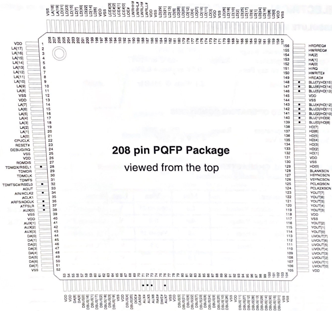
Figure 18. 208 QFP MPP Pinout
