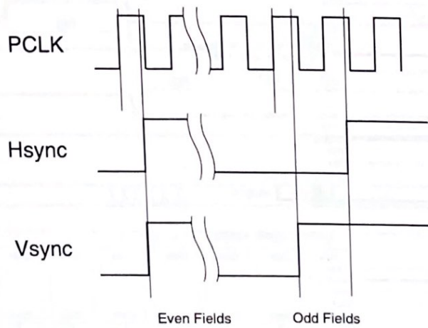
Figure 8. Odd/Even Video Output Timing
