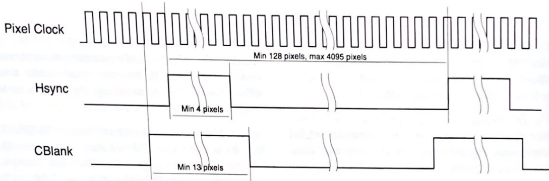
Figure 6. Horizontal Video Timing
