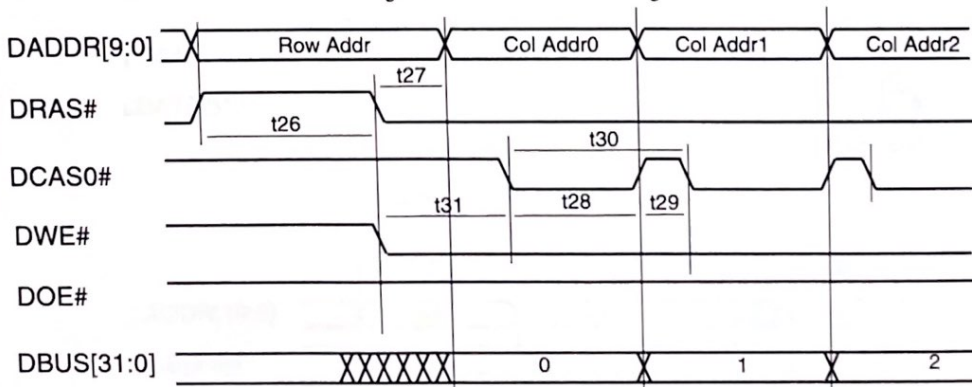
Figure 11. DRAM Write Timing
