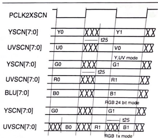
Figure 5. 1x Clock Video Out Bus Timing
