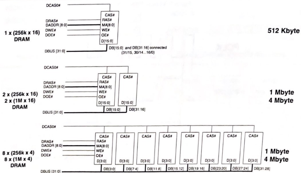
Figure 9. DRAM Configurations
