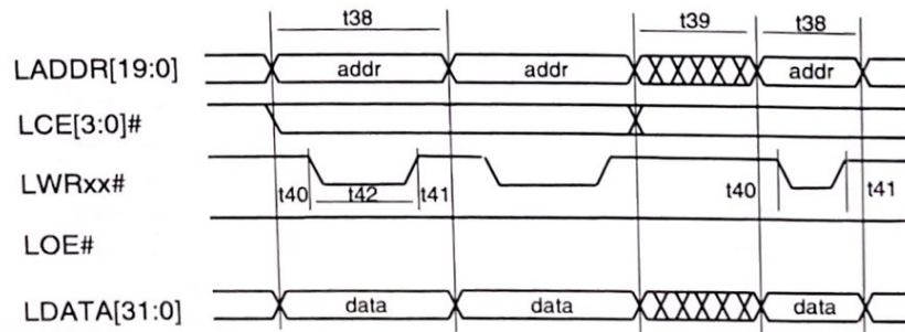
Figure 13. SRAM Write Timing
