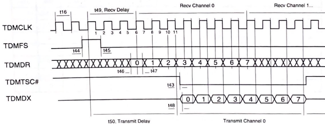
Figure 14. TDM Bus Timing
