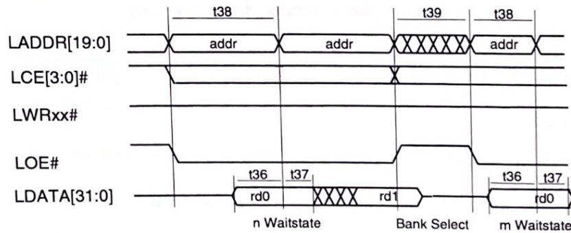
Figure 12. SRAM Read Timing
