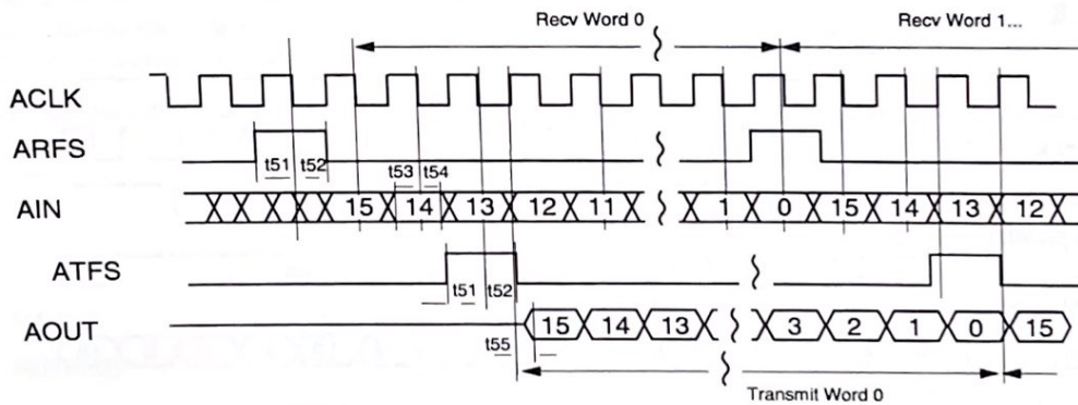
Figure 15. Audio Bus Timing
