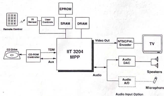
Figure 1. MPPex Stand-alone System
