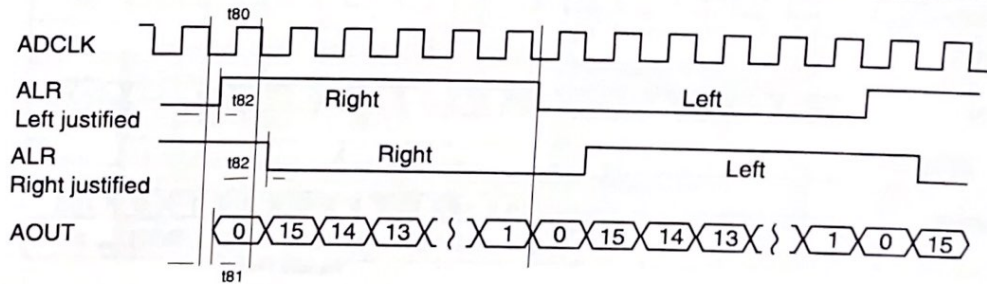
Figure 16. Decoder Mode Audio Port Timing
