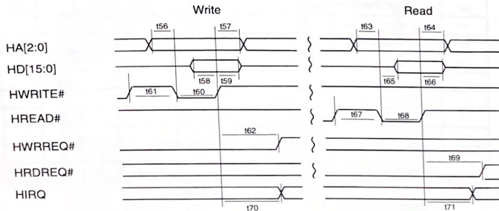
Figure 17. Host Bus Timing
