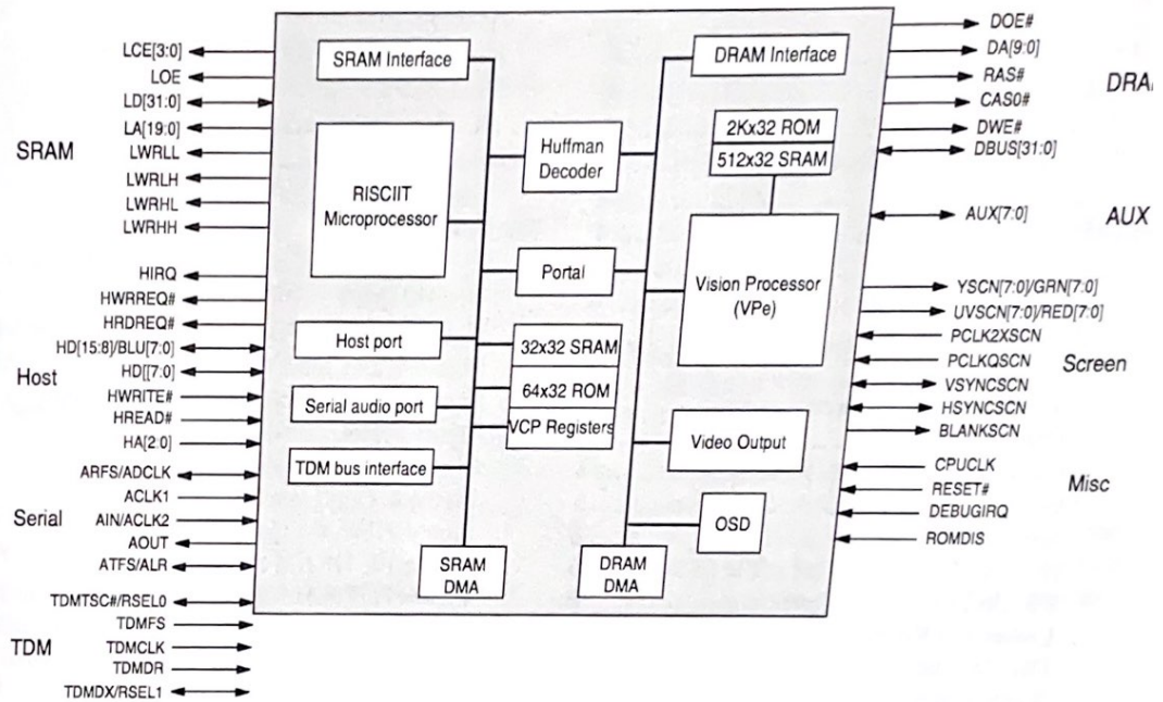
Figure 2. MPPex Block Diagram
