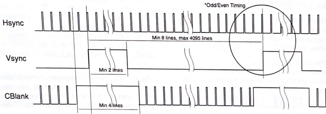
Figure 7. Vertical Video Timing
