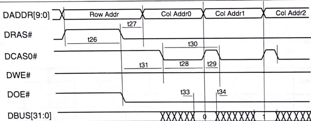
Figure 10. DRAM Read Timing
